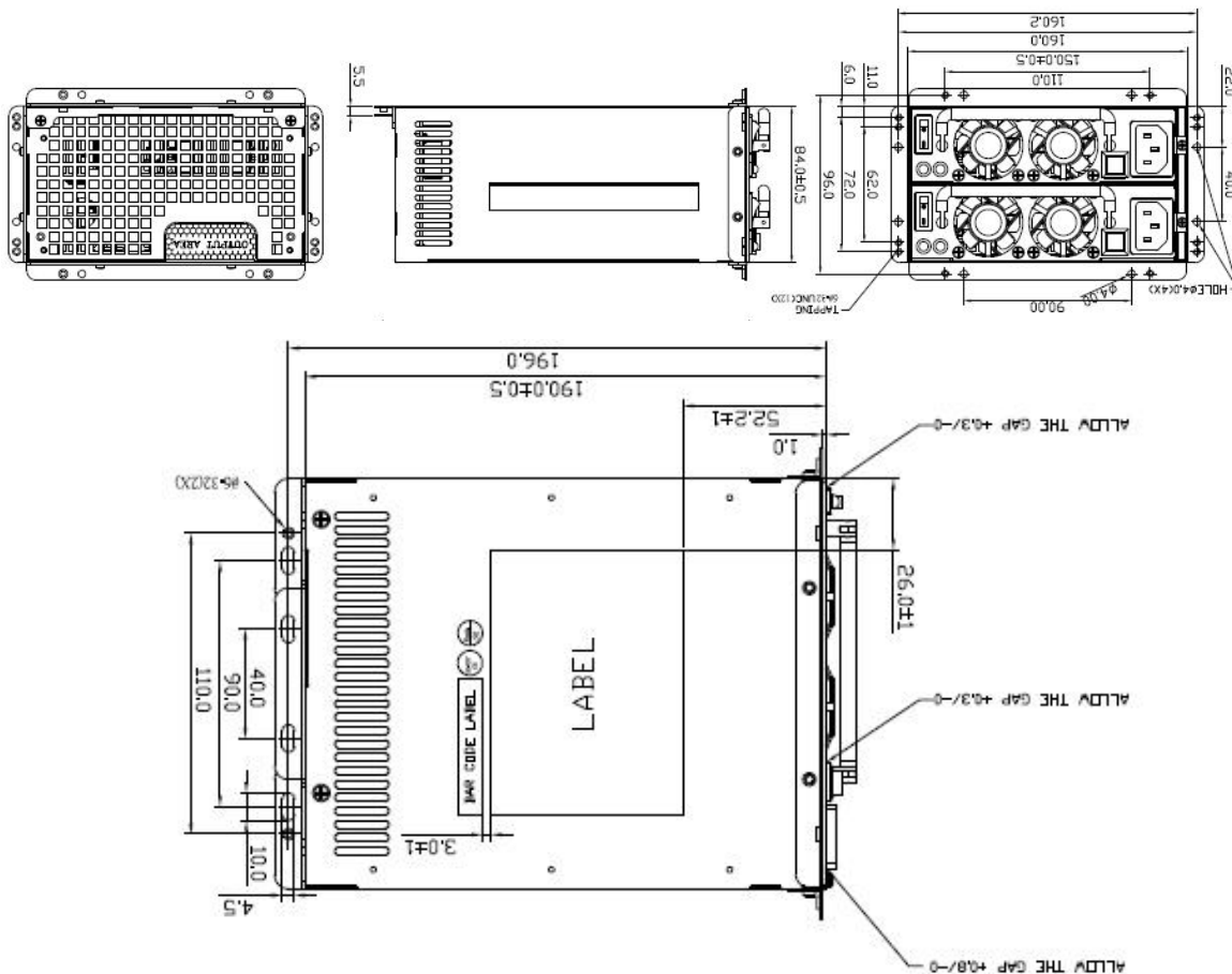
Figure 1: Cage Enclosure Drawing
