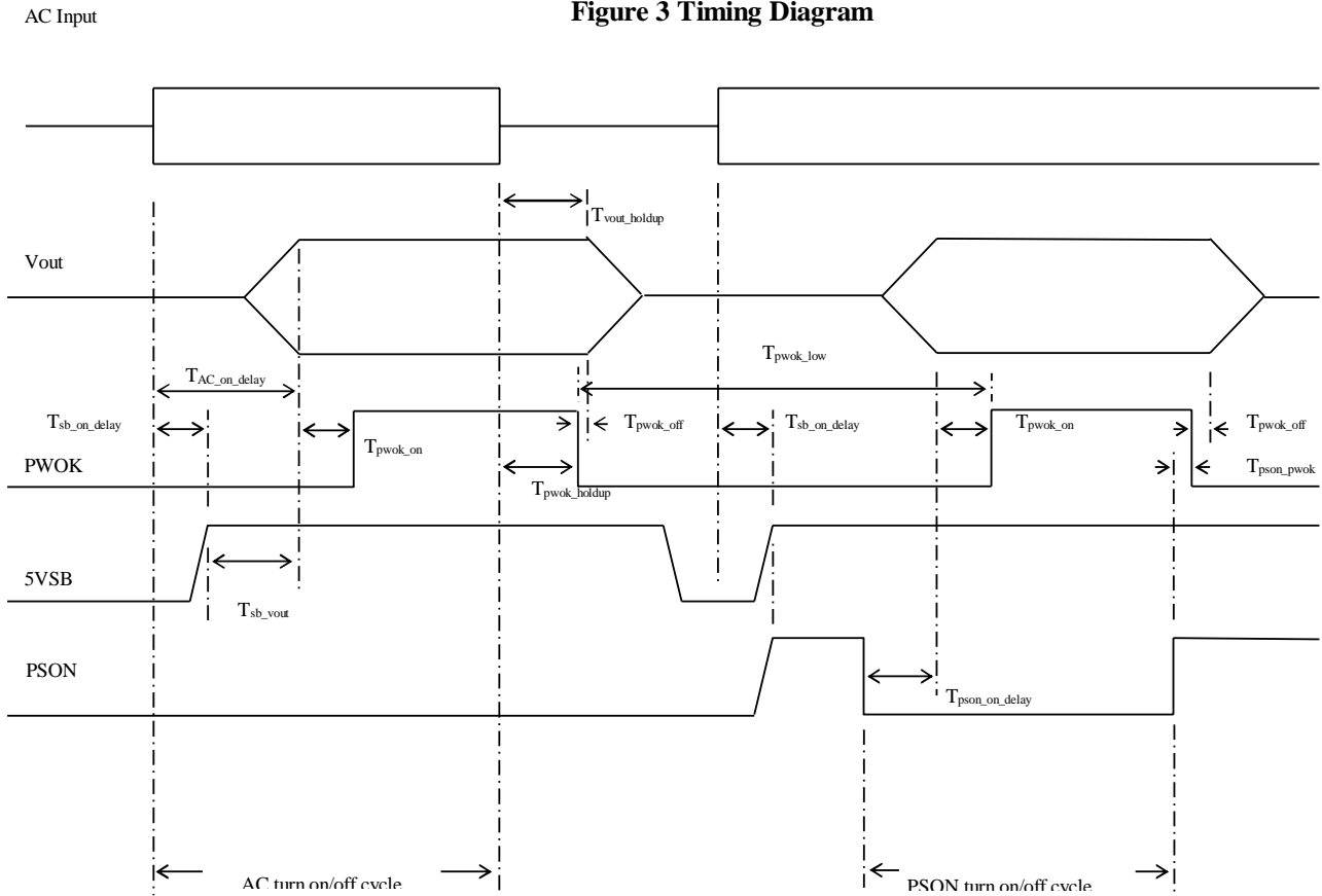
Figure 3 Timing Diagram
